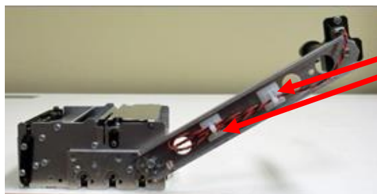
roll holder arm (P/N 424051-U)
